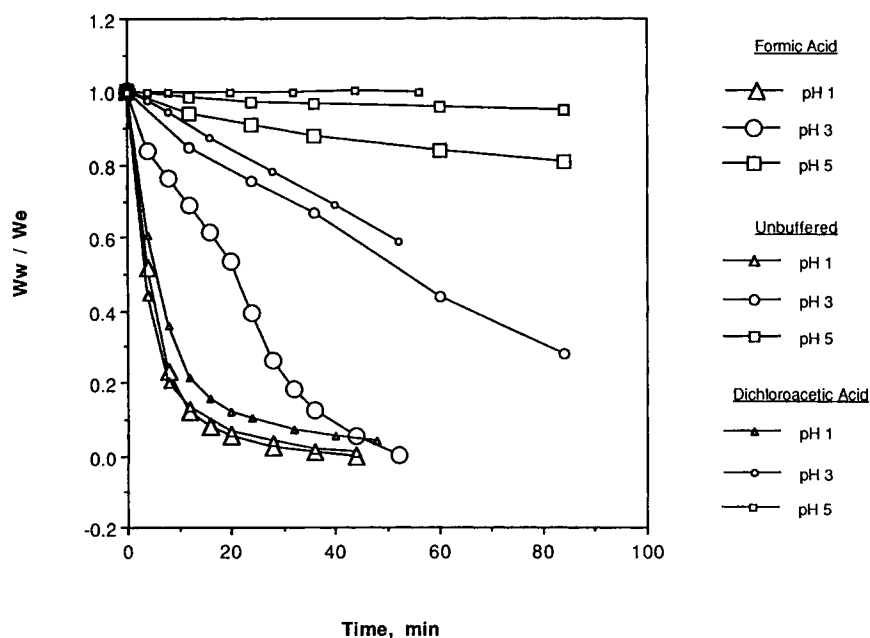
Figure 10 Comparison of deswelling kinetics for unbuffered, dichloroacetic acid, and formic acid at pH 1, 3, and 5; 78/22 mol % HEMA/MAA gel. Formic acid at pH 1 ( -\Delta- ), pH 3 ( -\circ- ), and pH 5 ( -\square- ); Unbuffered at pH 1 ( -\Delta- ), pH 3 ( -\circ- ), and pH 5 ( -\square- ); Dichloroacetic Acid at pH 1 ( -\Delta- ), pH 3 ( -\circ- ), and pH 5 ( -\square- ).
