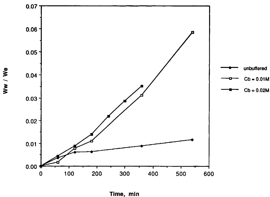
Figure 1 Comparison of swelling kinetics for buffered and unbuffered solutions; variation of total buffer concentration 78/22 mol % MMA/MAA gel; pH 9; Imidazole buffer used; Cb = total buffer concentration. (—◆—) Unbuffered; (—□—) Cb = 0.01M; (—□—) Cb = 0.02M.
