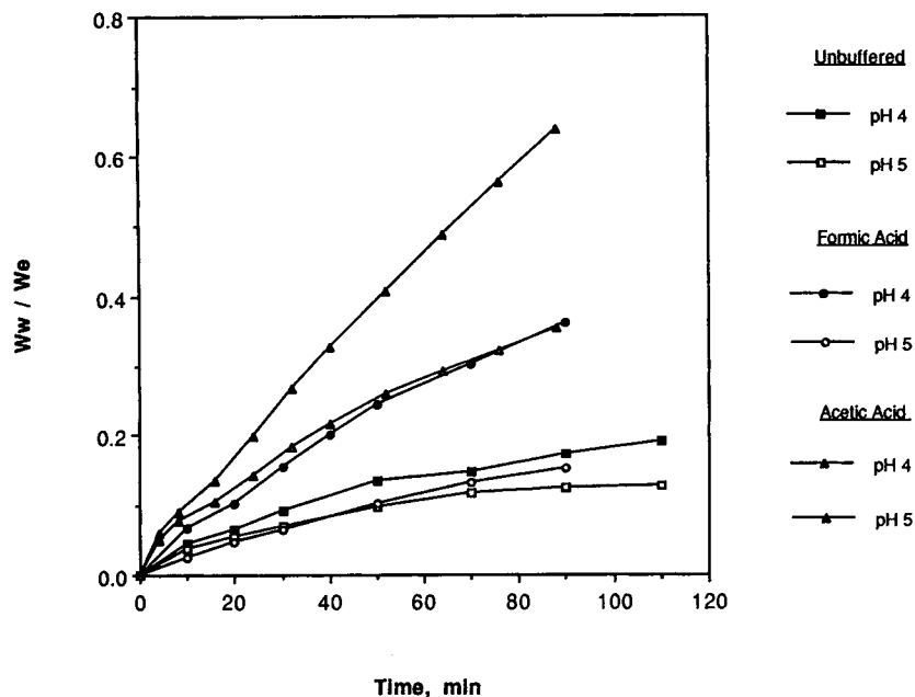
Figure 7 Comparison between swelling kinetics for unbuffered, formic acid and acetic acid at pH 4 and 5; 78/22 mol % HEMA/DMA gel. Unbuffered at pH 4 (—■—) and pH 5 (—□—); formic acid at pH 4 (—●—) and pH 5 (—○—); acetic acid at pH 4 (—▲—) and pH 5 (—△—).
