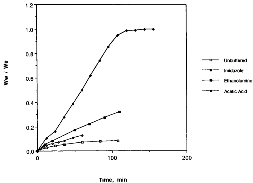
Figure 8 Comparison of swelling kinetics for amine versus carboxylic acid buffered solutions; 78/22 mol % HEMA/MAA gel; pH 9. (—□—) Unbuffered; (—◆—) imidazole; (—■—) ethanolamine; (—◇—) acetic acid.
