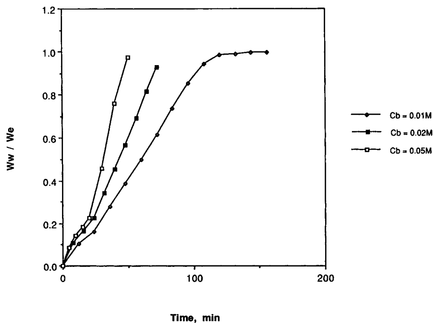
Figure 2 Variation of total buffer concentration for swelling kinetics; 78/22 mol % HEMA/MAA gel; pH 9; Imidazole buffer used; Cb = total buffer concentration. (—◇—) Cb = 0.01 M ; (—■—) Cb = 0.02 M ; (—□—) Cb = 0.05 M .
