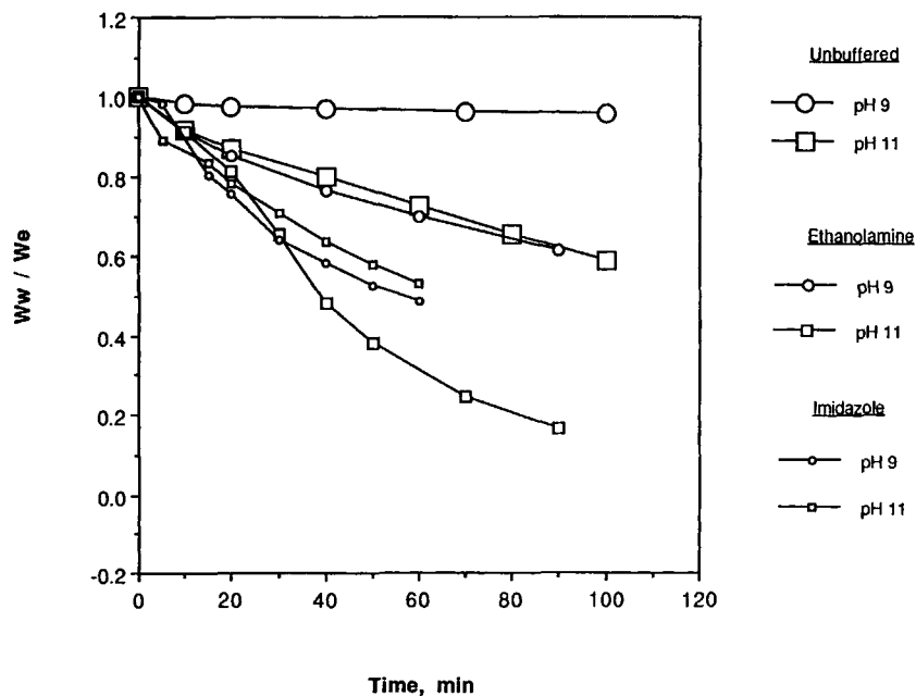
Figure 11 Comparison of deswelling kinetics for unbuffered, imidazole, and ethanolamine at pH 9 and 11; 78/22 mol % HEMA/DMA gel. Unbuffered at pH 9 (—○—) and pH 11 (—□—); ethanolamine at pH 9 (—○—) and pH 11 (—□—); imidazole at pH 9 (—○—) and pH 11 (—□—).
